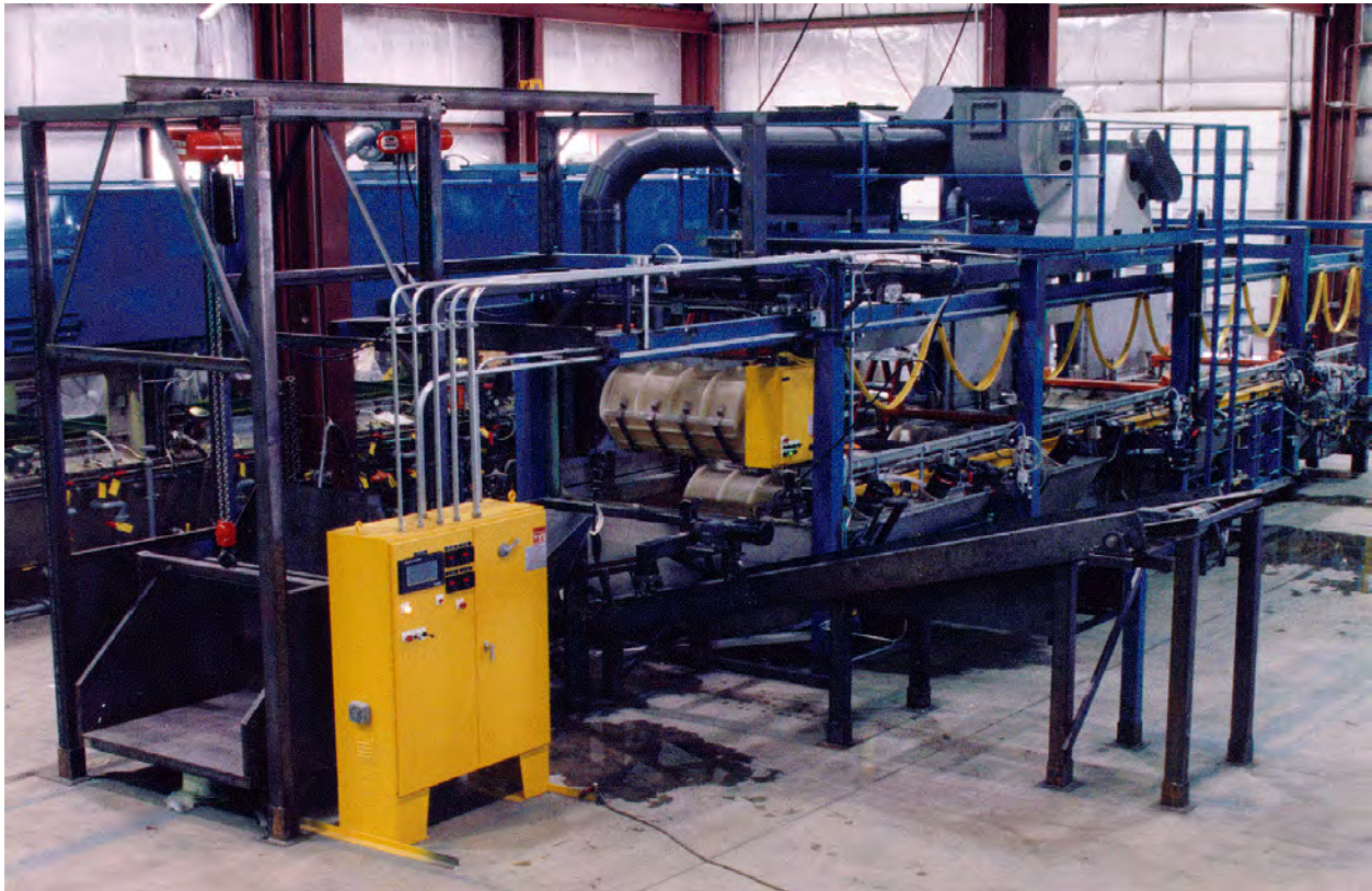
Figure 4. Example of a programmed hoist system. This system has a single, multi-speed traveling hoist for load transfers.
